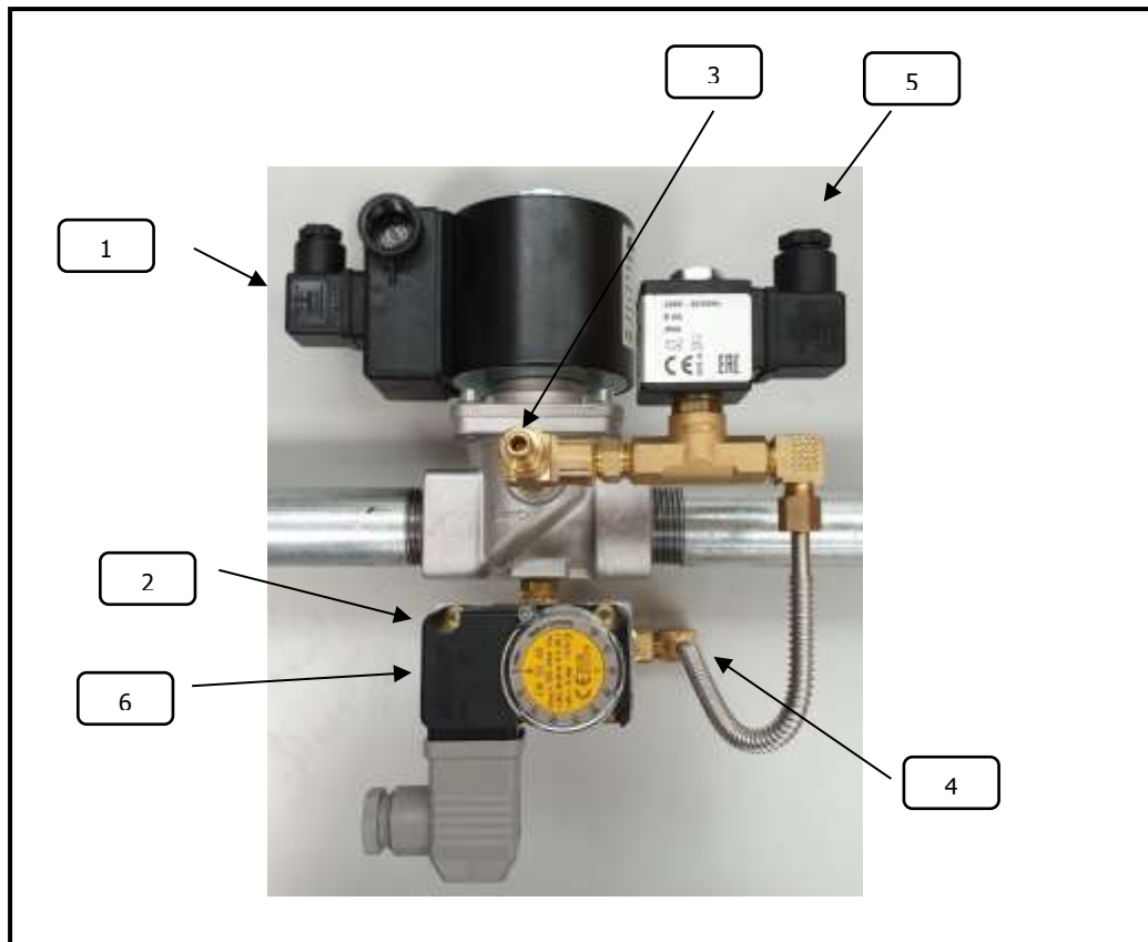
Figure 1b – Gas Train Components
