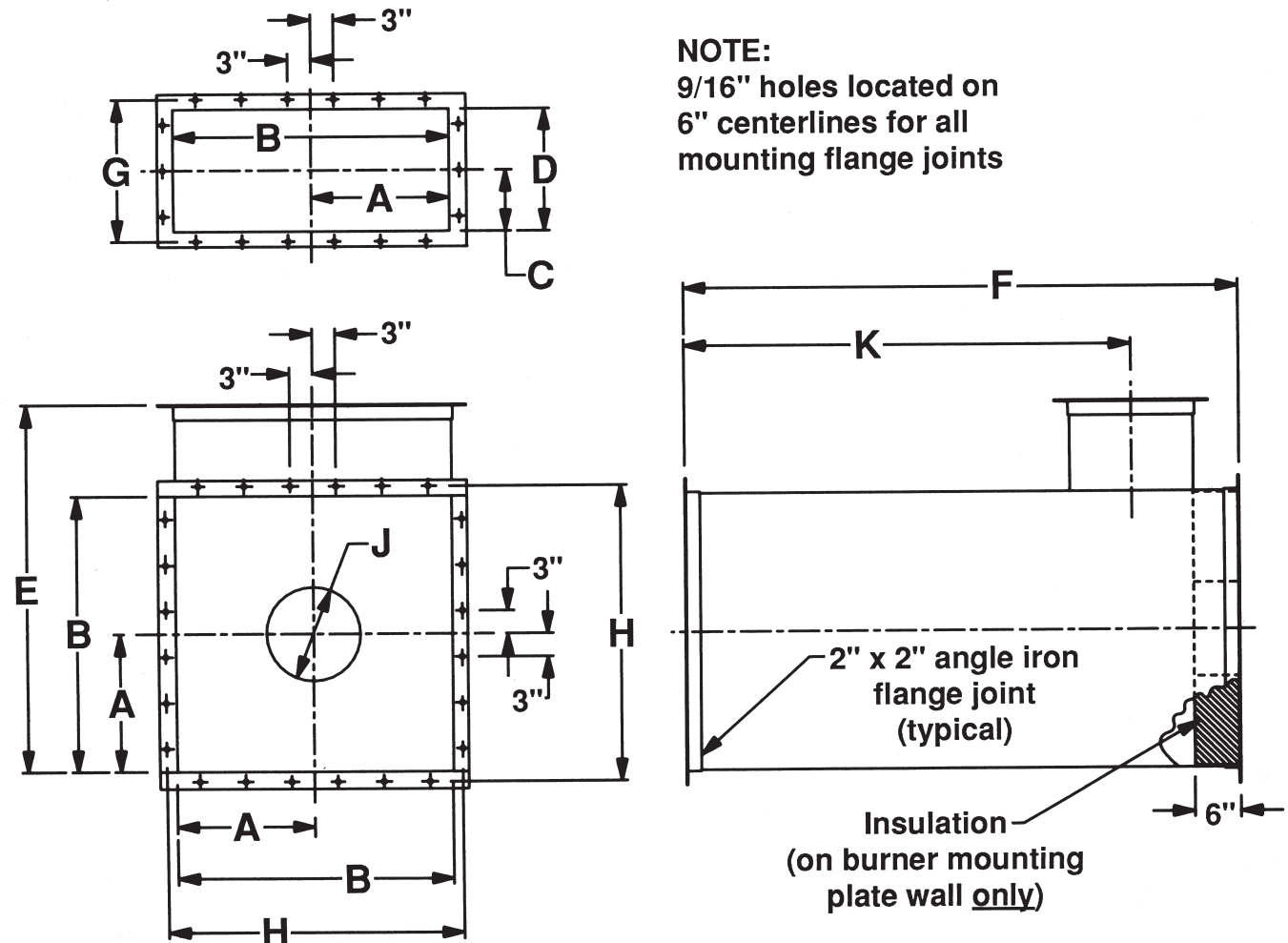
Approximate duct section dimensions (in inches)
