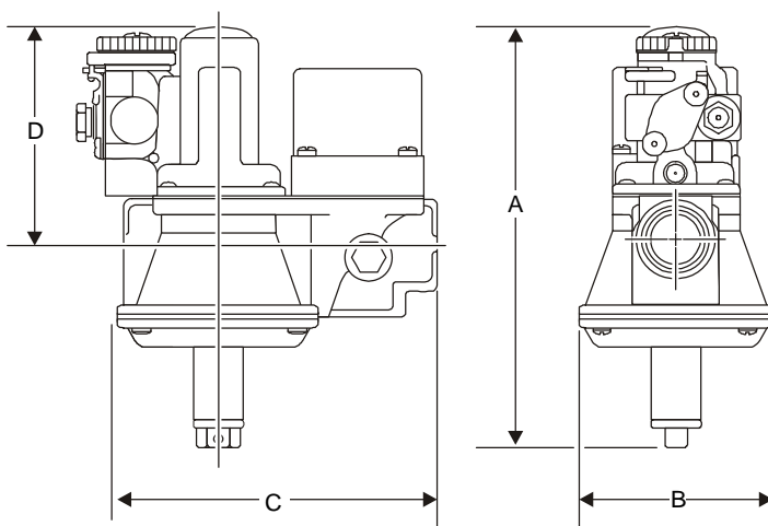
Figure 5: Direct-acting Regulator Model Dimensions
