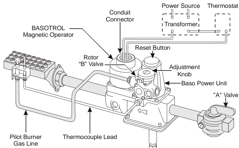
Figure 2: Typical Installation Showing Internal Pilot Gas Flow and Rotor "B" Valve
