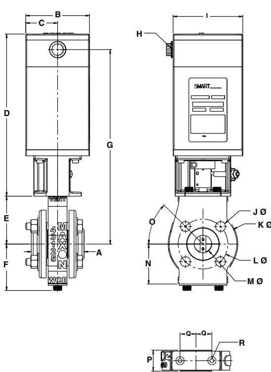
1" SMARTLINK® Butterfly Valve
