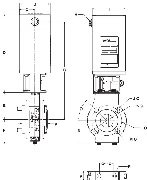
1.5" SMARTLINK® Butterfly Valve
