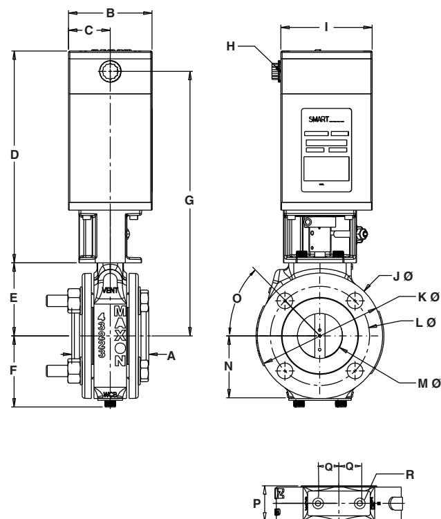
2" SMARTLINK® Butterfly Valve
