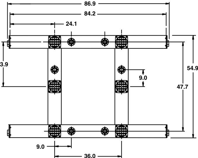
7 BI XF GRD with 48" span
